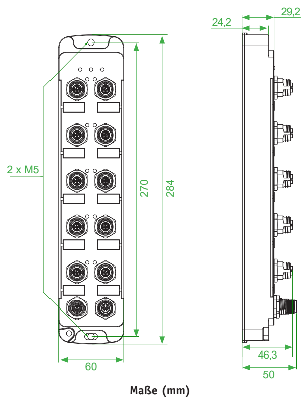
PROFINET Switch PROmesh P10X
